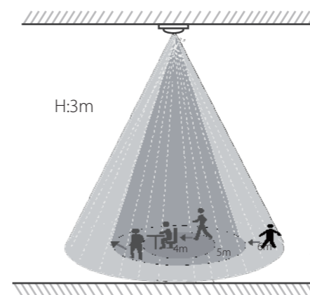
Ultrasonic Detection Range
